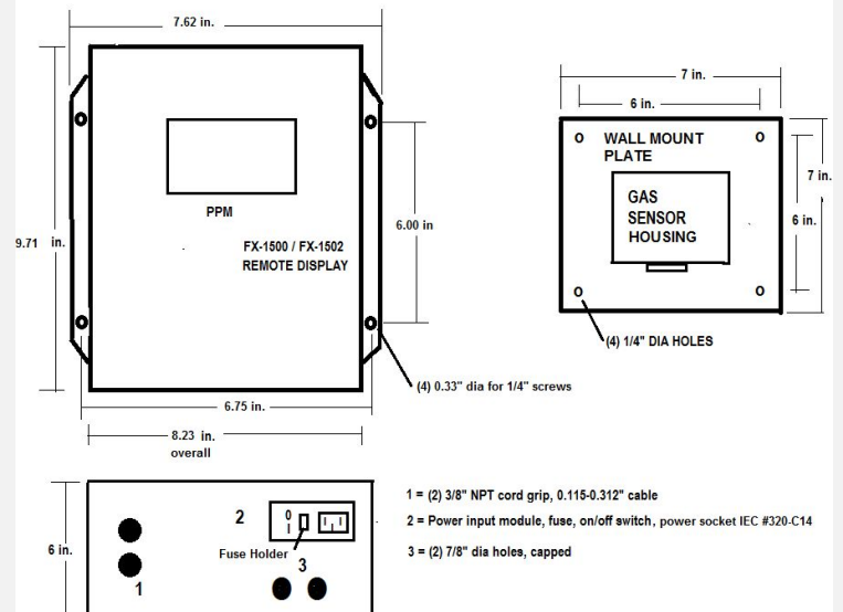
Foxcroft FX-1500v4 & FX-1502v4 Gas Detectors Dimensions
